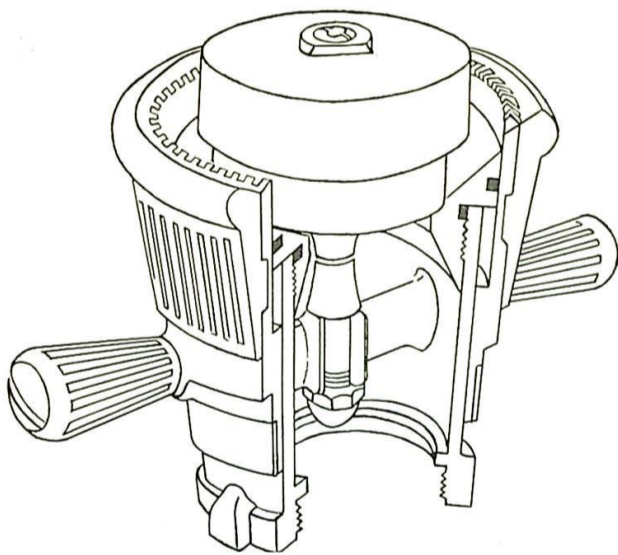
The Task Force Tip . Note compact automatic cylinder-baffle mechanism in center of business end of conventional constant-volume fog tip.
