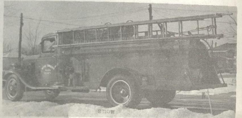
The 500 gpm pumper built by volunteers in 1942 as a second pump, in order for them to gain a Class A rating. Materials were so scarce at that time the entire bed and shell behind the cab was constructed of plywood.
